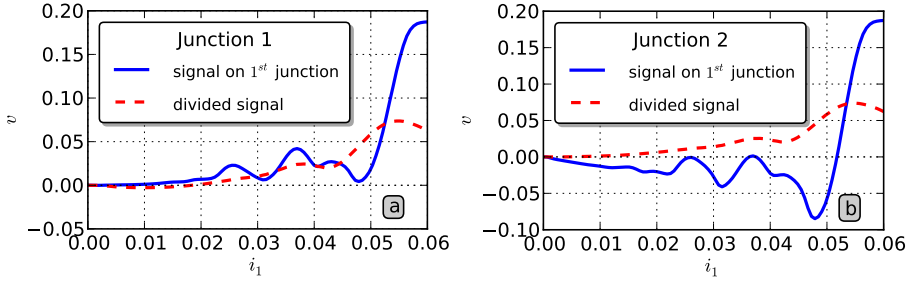
Fig. 5. (Colour online) The long-time averaged voltage v across the first panel (a) and the second panel (b) junction. The panels show the dependence on the DC bias I_1 at fixed temperature D = 2 \times 10^{-5} for two different types of driving, i.e. applied to only one junction ( a_1 = 1.775, a_2 = 0 , solid/blue line) and applied to both of them ( a_1 = 0, a_2 = 1.775 , dashed/red line). Other parameters are coupling strength \alpha = 0.77 , the frequency of the AC driving \omega = 0.1875 .
